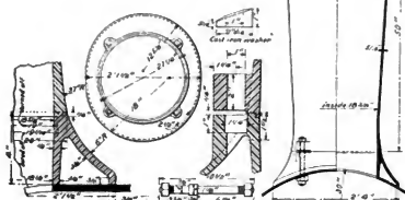
Figs. 458-463. Cast-Iron Taper Stack. Six-Wheel (0-6-0) Switching Locomotive. Baltimore & Ohio.
